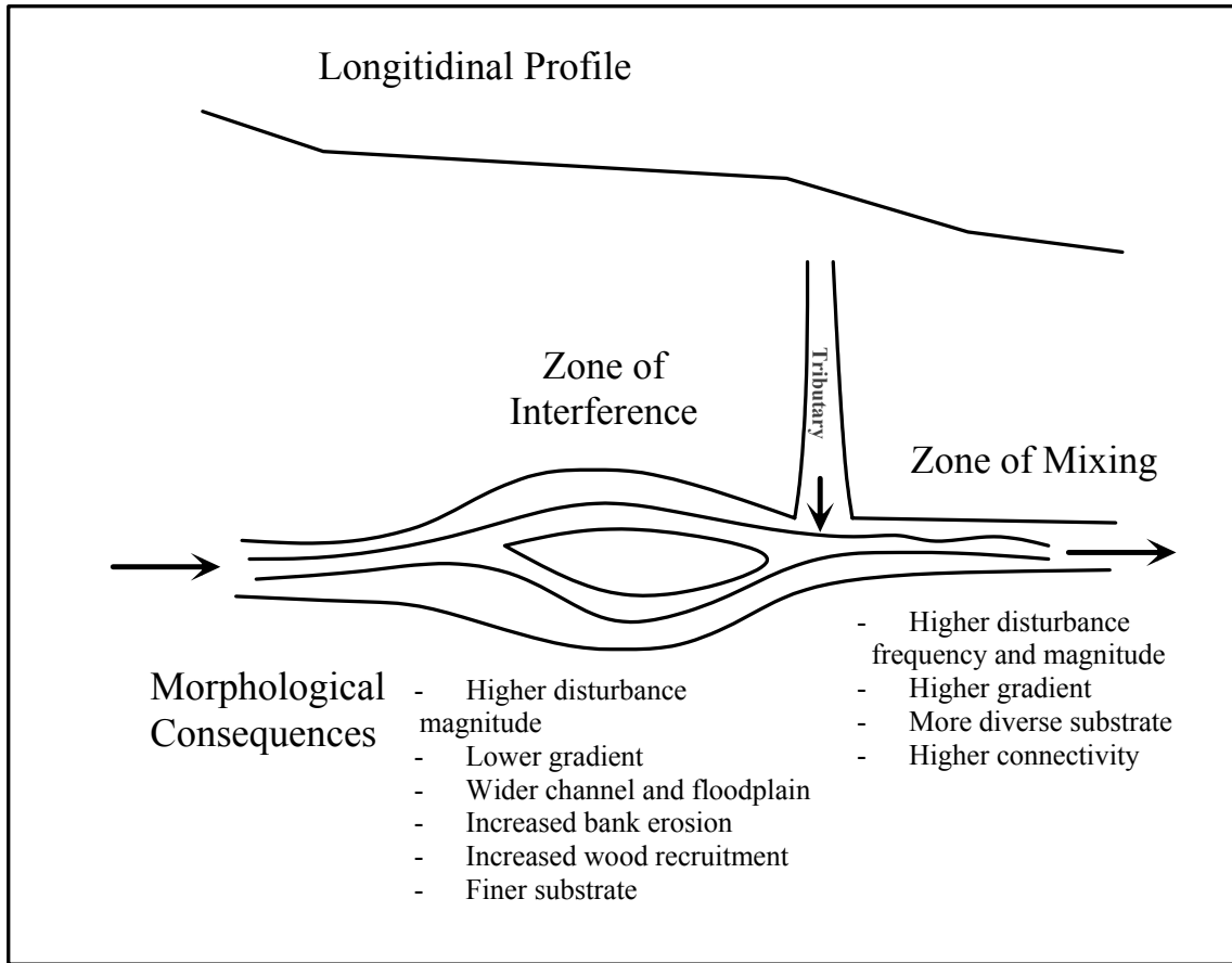
Figure 8. Large influxes of sediment from tributary basins in Idaho affected the morphology of the receiving channel in proximity to rejuvenated alluvial fans (e.g., Figure 2, A). Effects upstream of fans include decreases in channel slope, increases in floodplain width, decreases in substrate size, increases in side channels, and terrace rejuvenation. Effects downstream of fans include channel steepening and boulder-dominated cascade morphology. Increased channel instability may also lead to greater lateral connectivity between channels and their floodplains and terraces, and hence increased wood recruitment. The zone of fan influence may expand during large sedimentation events and contract during periods of low watershed disturbance.
