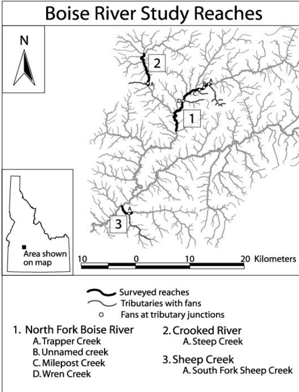
Figure 1. Twenty-seven kilometers of river in the Boise River basin were surveyed to document the effects of punctuated erosion following the Rabbit Creek fire (1995) on alluvial fans and channel morphology.
