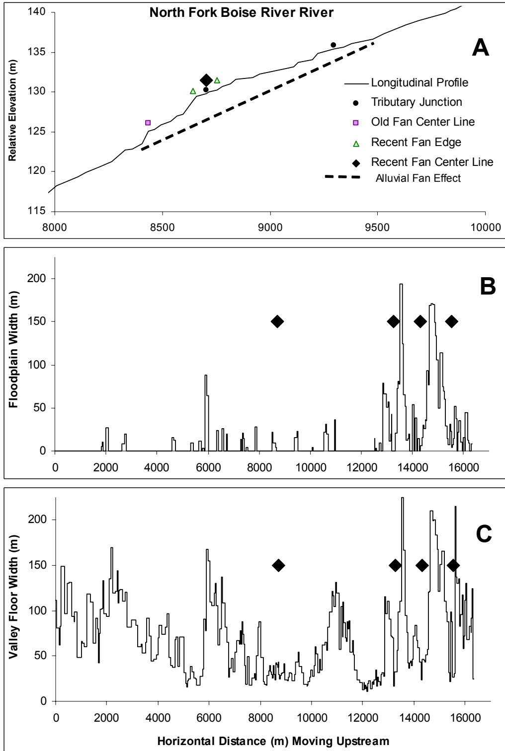
Figure 5. (A) Longitudinal profile of North Fork Boise River (drainage area 220 km 2 ) showing a step caused by the rejuvenated alluvial fan from Wren Creek (11 km 2 ). The
