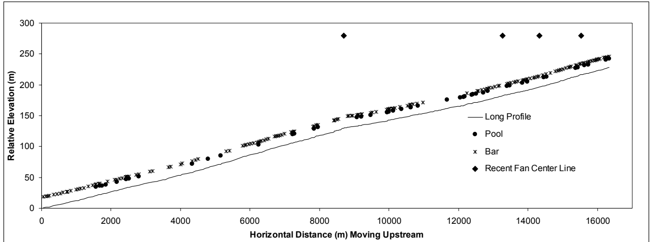
Figure 7. Number and location of large pools (> 1m residual depth) along 16 km of the North Fork Boise River in relation to recently active alluvial fans.
